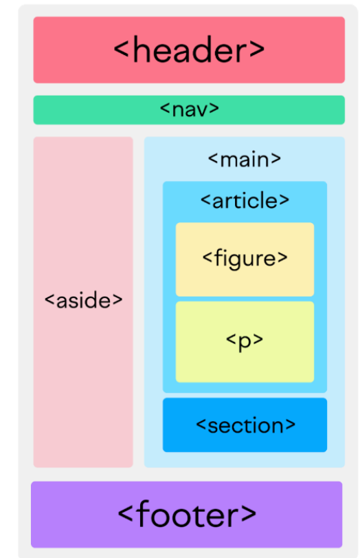
Semantic HTML
