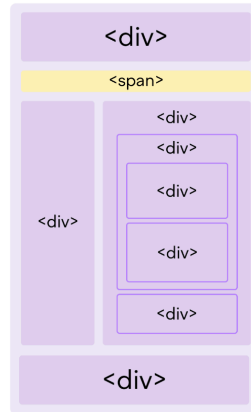
Non-Semantic HTML
